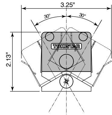
Adjustable Bracket Securely attach with screws.
